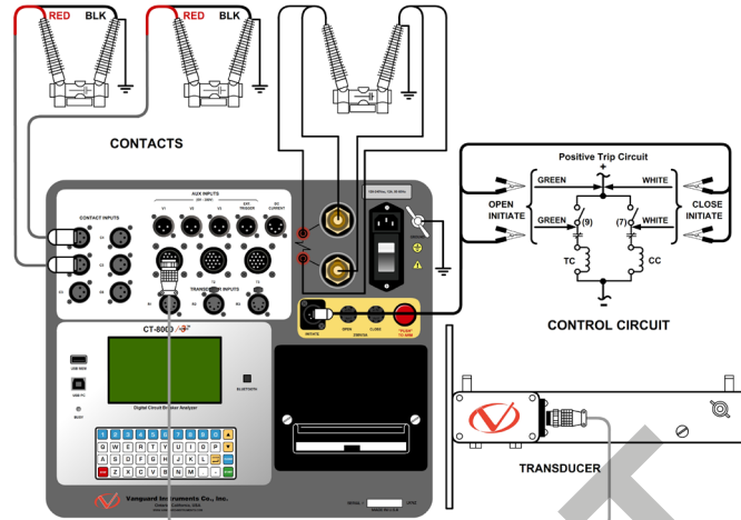
Typical CT-8000 S3 Dynamic Resistance Test Connections
