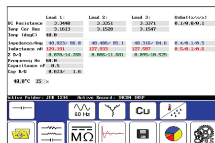
RLC measurements screen.
