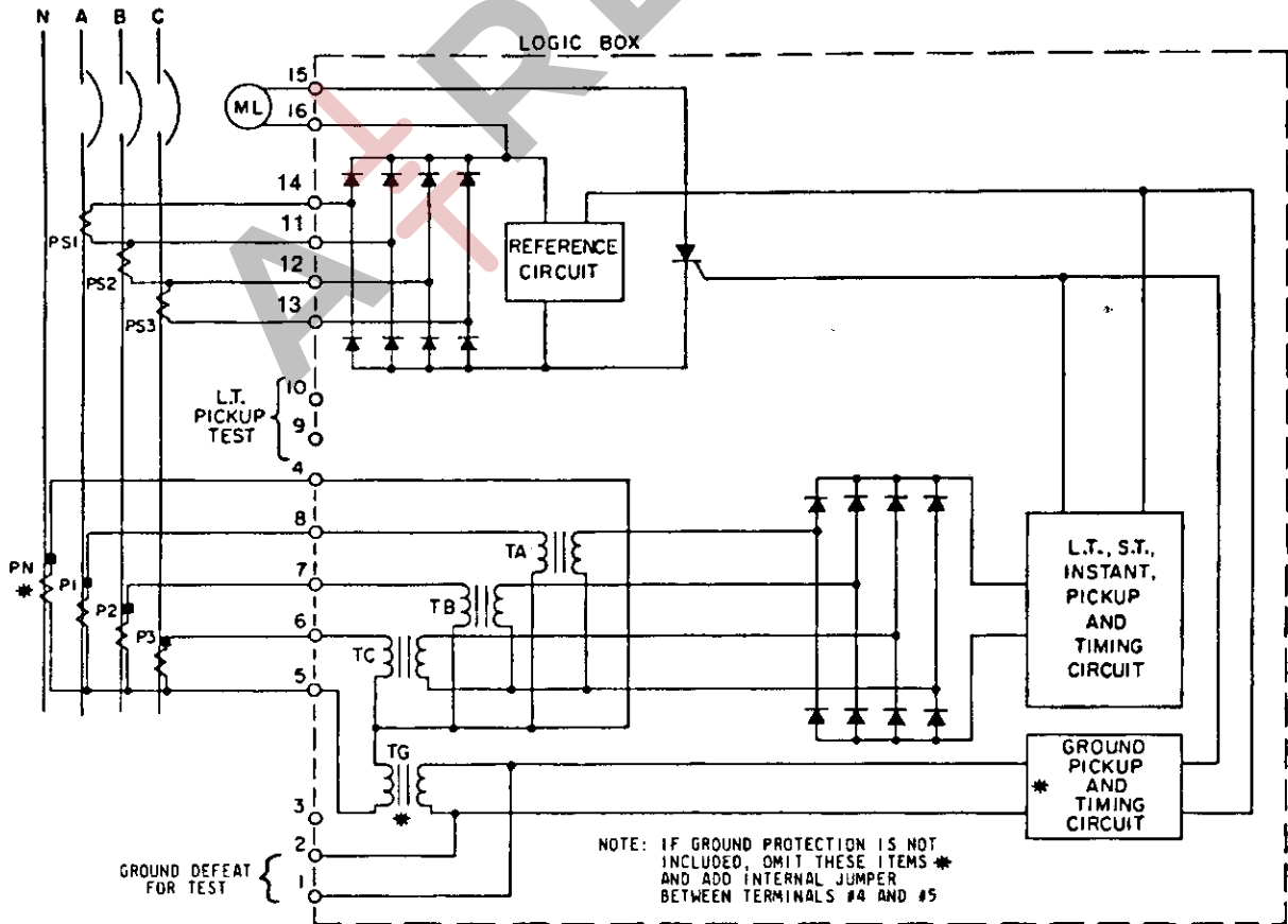
Fig. 3 — Typical Wiring Diagram of Standard 3- or 4-Wire System with Ground Fault Protection
