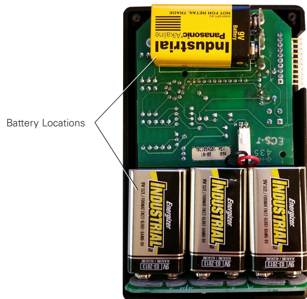
Figure 3. Battery Locations.
