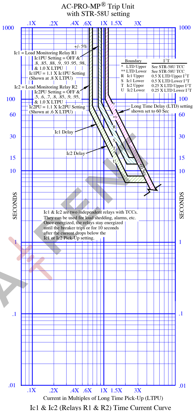
Figure 10 AC-PRO-MP STR-58U Load Monitoring Time-Current-Curve
