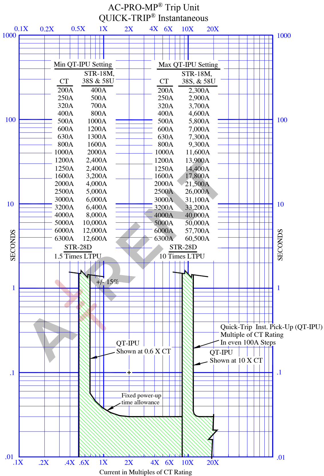
Figure 11 AC-PRO-MP Quick-Trip® Instantaneous Time-Current-Curve
