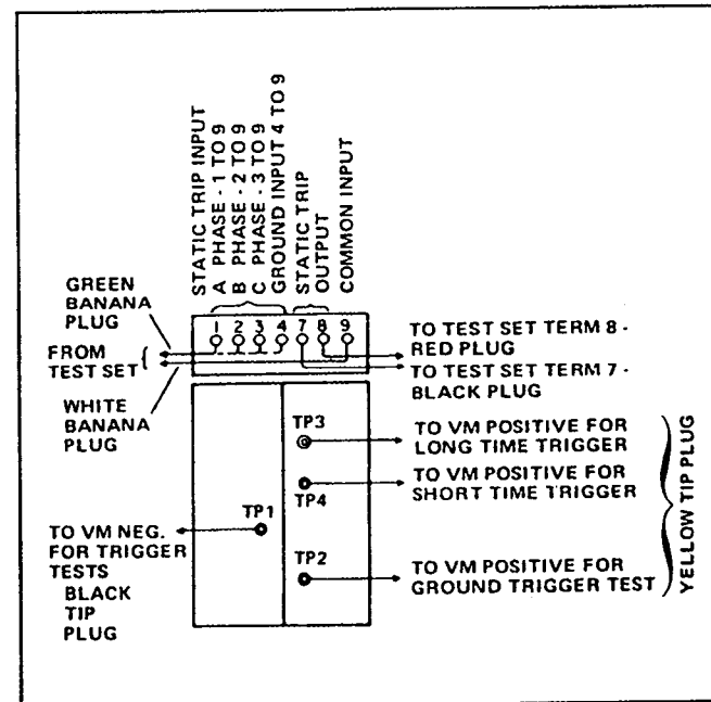
Figure 11. Testing With Portable Test Set, Connection Diagram
