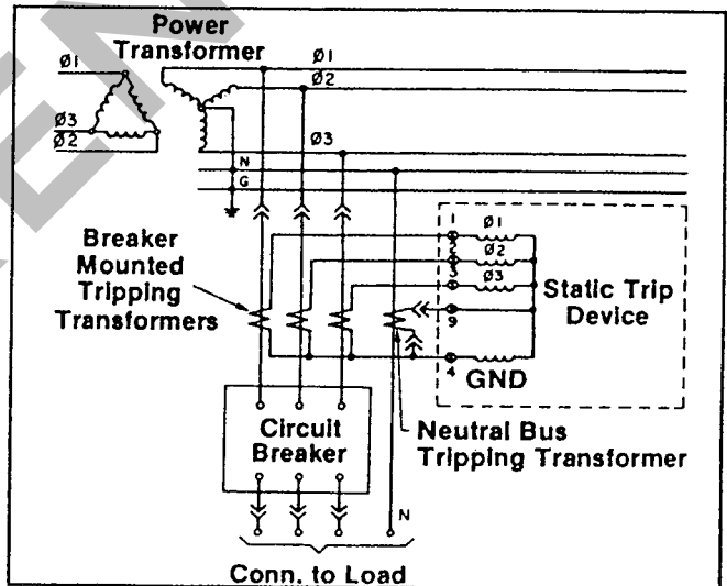
Figure 6. Breaker Wiring for Ground Protection on 4-Wire Systems, Residual Sensing
