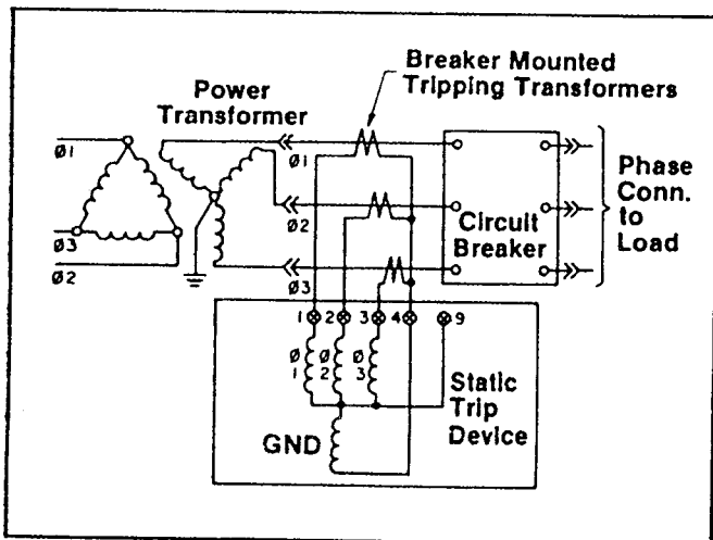
Figure 5. Breaker Wiring for Ground Protection on 3-Wire Systems, Residual Sensing
