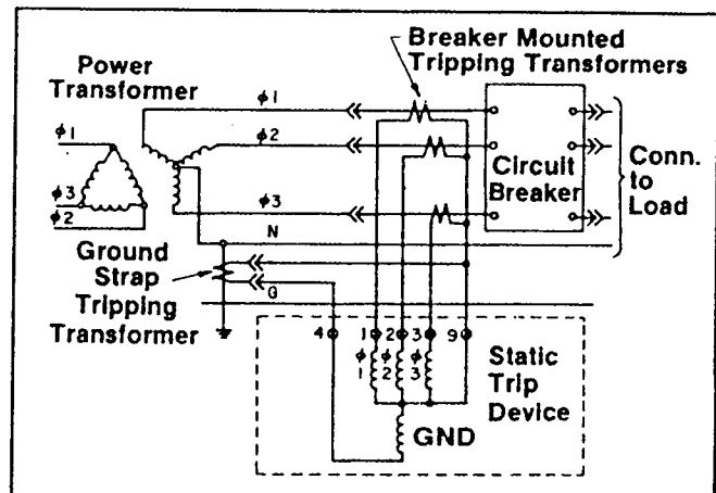
Figure 7. Breaker Wiring for Ground Protection on 4-Wire Systems, Ground Strap Current Sensing
