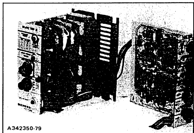
Figure 14. Static Trip II Disassembled
