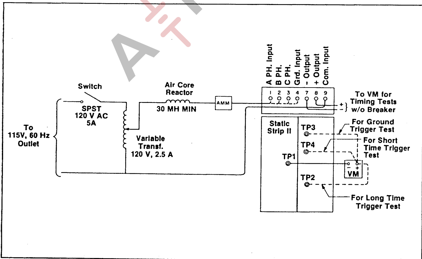
Figure 12. Secondary Testing Without Test Set
